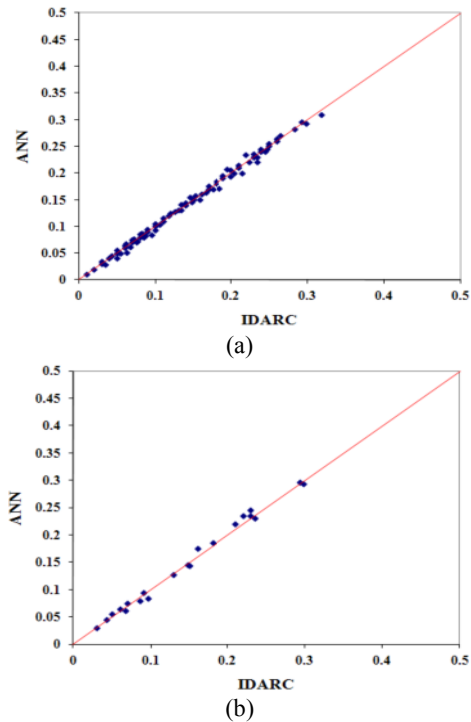
Fig. 4 Performance of proposed ANN model: (a) training set and (b) testing set
