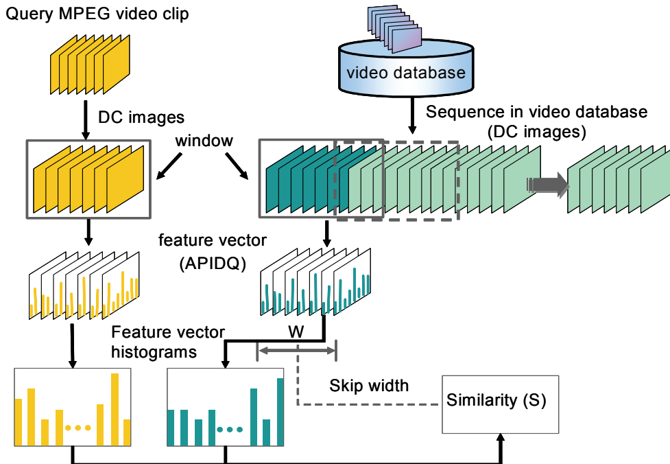
Fig.2 The procedure of proposed fast search algorithm.
