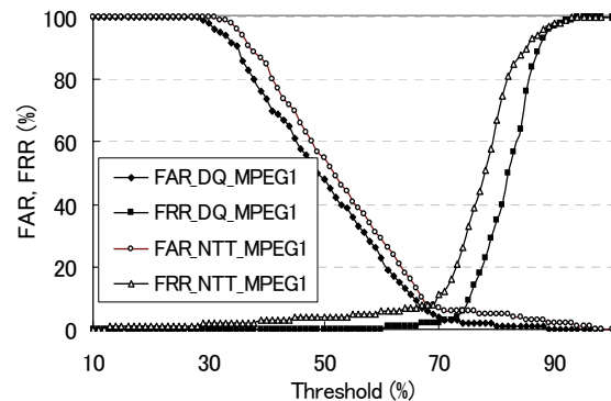
Fig.4 Comparison of FAR and FRR (DC images).
