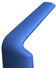
Fig. 11: Geometry of the first analyzed winglet
