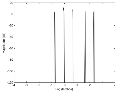
Fig. 1 MUSIC pseudospectrum of S_1(\tau) with SNR of 40dB
