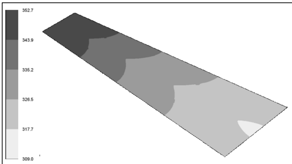
Fig. 13 Temperature contours of absorber plate for dimple plate collector at 1000W/m 2
