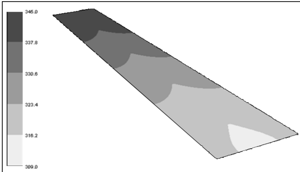
Fig. 12 Temperature contours of absorber plate for flat plate collector at 1000W/m 2
