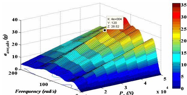
Fig. 14 Absolute average of deceleration of occupant submitted to cosine excitation for Dodge Neon
