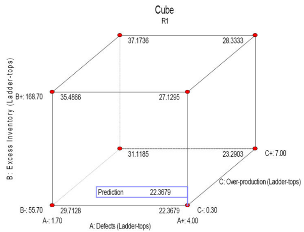
Fig. 14 Design expert8 cube plot depiction of optimum (MINIMUM) cost of wastes when D = 390.70
