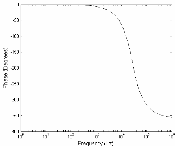
Fig. 7. PSPICE simulation results for the proposed multifunction filter showing all-pass phase response.
