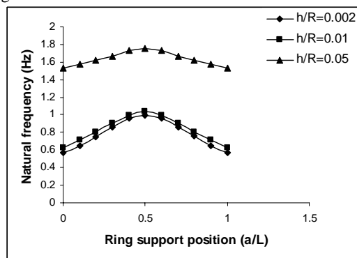
Fig. 6: Variation of the natural frequencies FG cylindrical shell with the position of the ring support a/L at different h/R ratios for C-C boundary conditions. ( m=1 , n=10 , L/R=20 )
