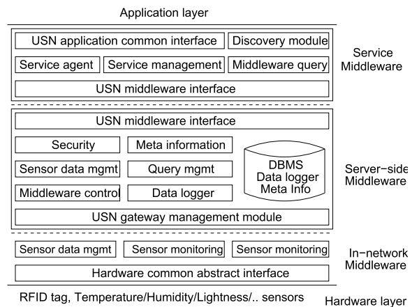
Fig. 1. USN middleware architecture
