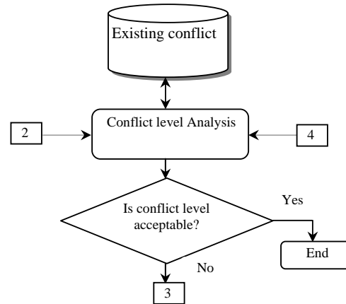
Fig. 3. Conflict level analysis.
