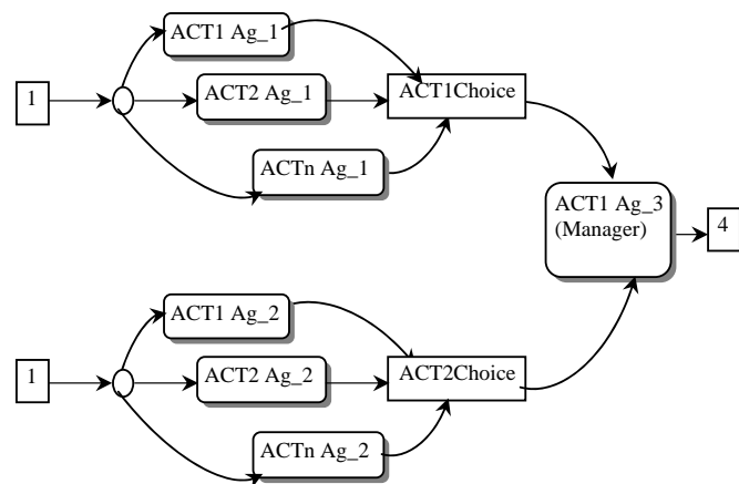
Fig. 5. Petri nets and scope boundaries.
