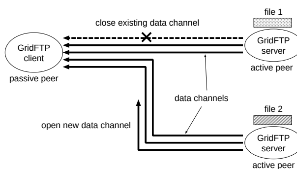
Fig. 2: Dynamic data channel allocation using the dynamic resource allocation: GridFTP v2 can adjust the number of data channels using READY/CLOSE/BYE commands during file transfer.
