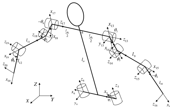
Fig. 3 Upper extremity of the humanoid robot
