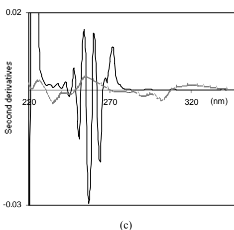
Fig. 1 The absorption spectra of PSE (600 \mu g/ml), (— line) and TRI (30 \mu g/ml), (---- line); (a) zero-order (b) first derivative and (c) second derivative
