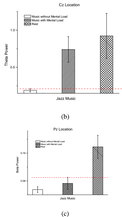
Fig. 3 Shows mean and one SEM of (a). Alpha power at C_z (b). Theta power at C_z (c). Beta power at P_z at three different experimental conditions for the entire subjects during jazz music
