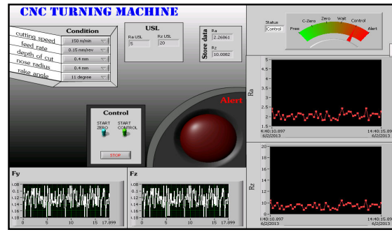
(a) In-process control of predicted surface roughness in turning process
