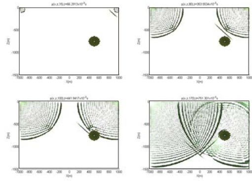
Fig. 7 Four subsequent snapshots of reflection seismic waves to investigate the locus of all possible underground scatter points centered at (500,-750) with the radius of 100\text{m} and r=0.999 .
