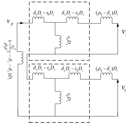
Fig. 2 MD Kirchhoff circuit representation of the 2D seismic system.
