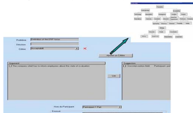
Fig. 5 DyPKM interface
