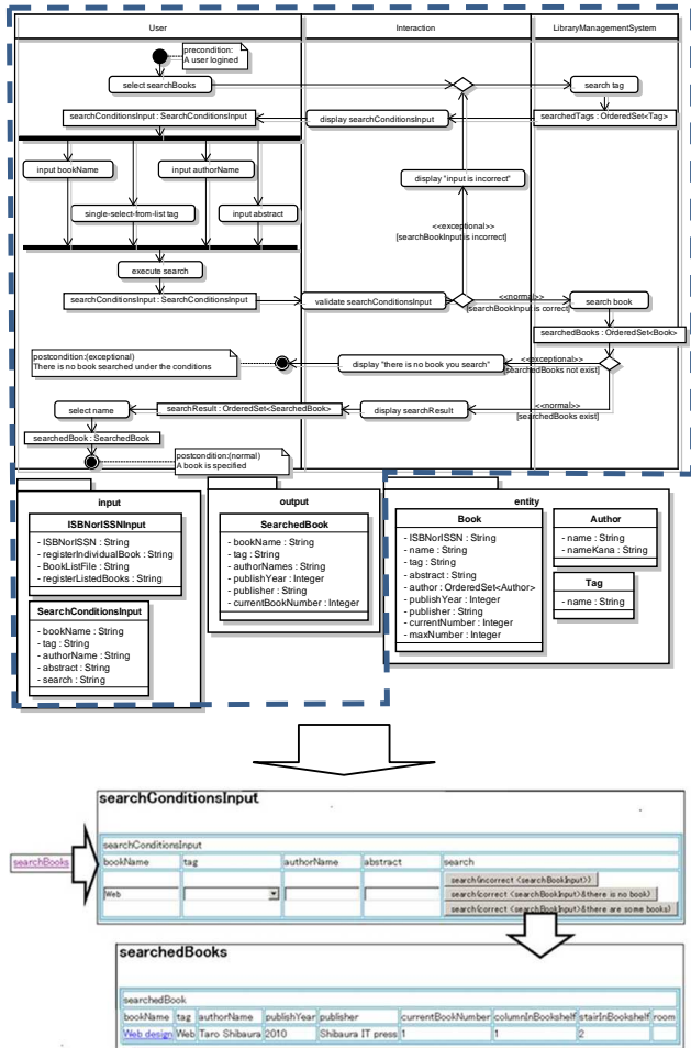
Fig. 1 UI mock-up generation from RA model
