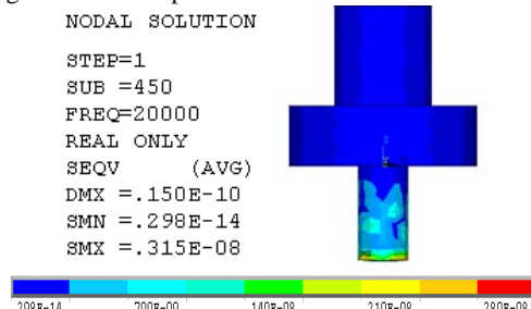
Fig. 3 Von mises stress produced in the tool
