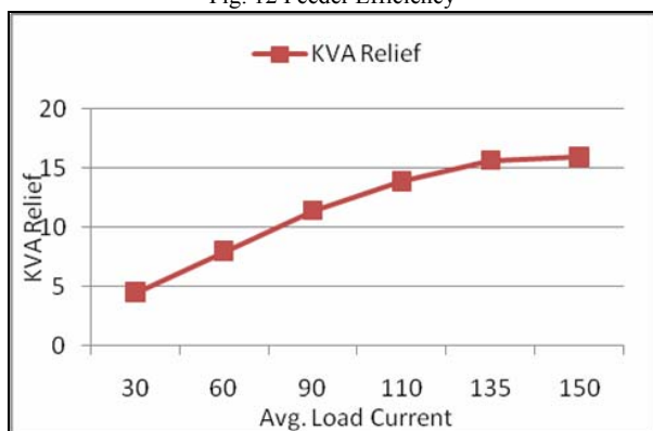
Fig. 13 KVA Relief with SVC
