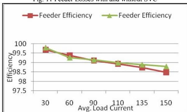
Fig. 12 Feeder Efficiency
