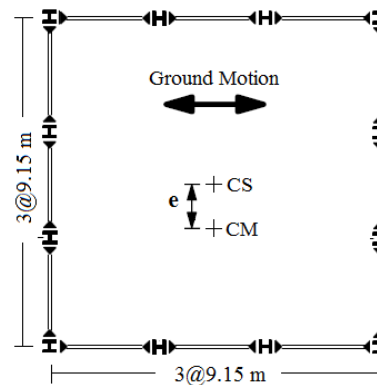
Fig. 2 The unsymmetric-plan building
