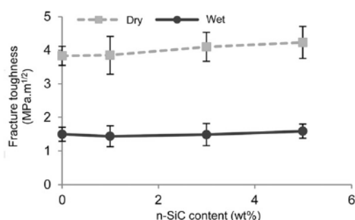
Fig. 16 Fracture Toughness of n-SiC filled RCF/epoxy eco-Nano composites for dry and wet conditions [4]
