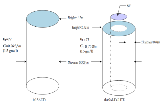
Fig. 4. Human body Models.
