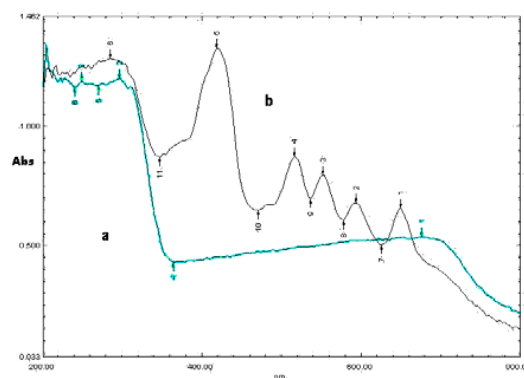
Fig. 5 Absorption spectra of \text{H}_2\text{TCPP} , a-before b-after sol-gel polycondensation
