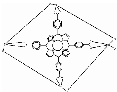
Fig. 3 Structure of Titanium gel doped with TCPP
