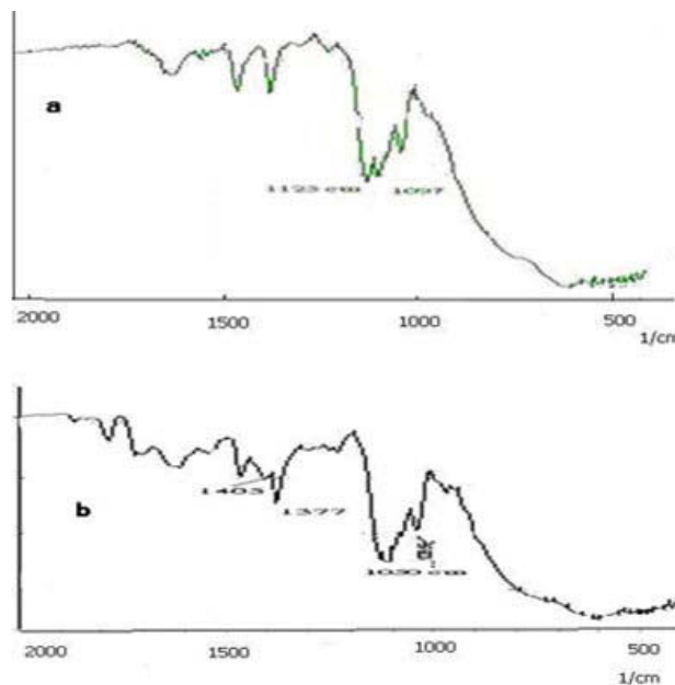
Fig. 4 a- Titanium gel, b-TCPP doped in gel
