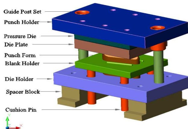
Fig. 3 Components of Non-Symmetry Drawing Die
