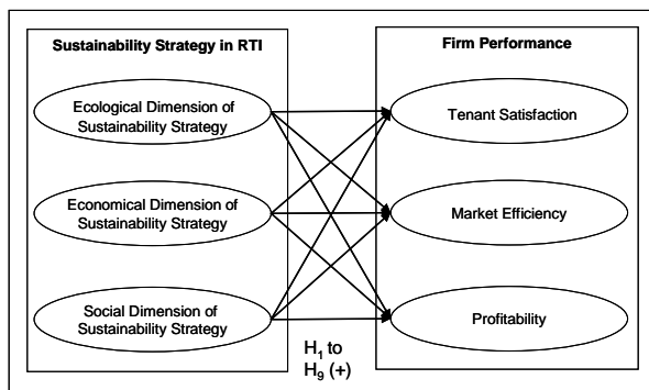
Fig. 1 Conceptual Framework
