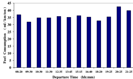
Fig. 4 Fuel consumption variation according to departure time
