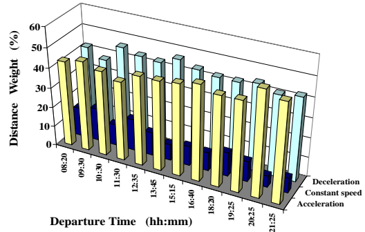
Fig. 7 Distribution of distance
