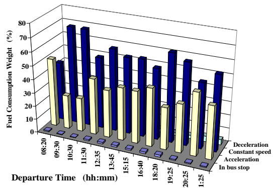
Fig. 11 Distribution of fuel consumed to characteristic processes for MODE 1 and MODE 2
