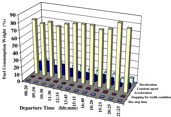
Fig. 6 Distribution of fuel consumed to the acceleration, constant speed, deceleration and stopping period
