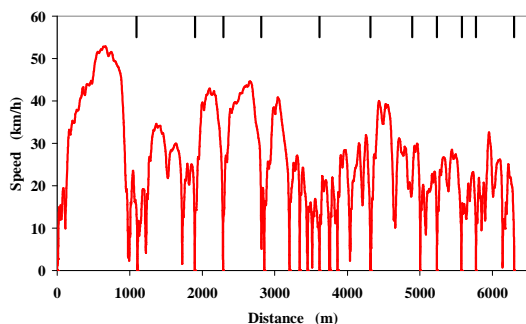
Fig. 3 Time - Distance trajectory of 19:25 trip
