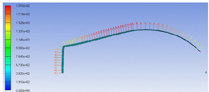
Fig. 15 Velocity vectors obtained from Autodyn at time = 0.045 msec
