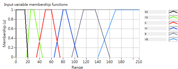
Fig. 9 Membership functions for the first input
