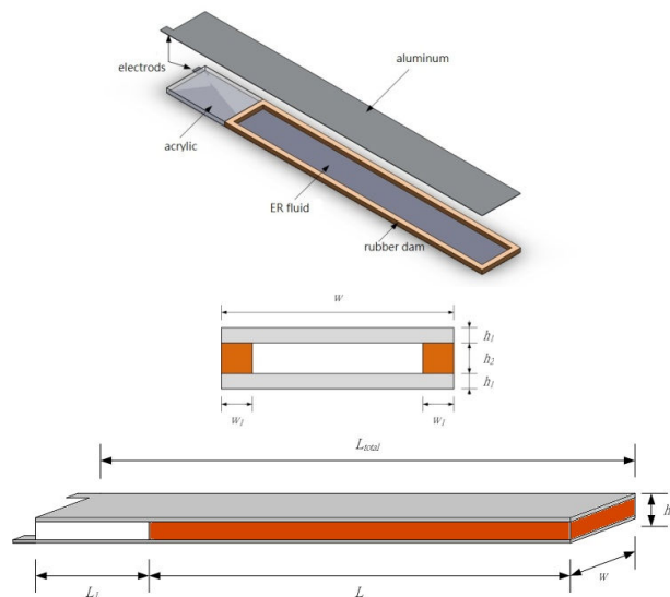
Fig. 1 The structure diagram and dimension of the ER sandwich beam
