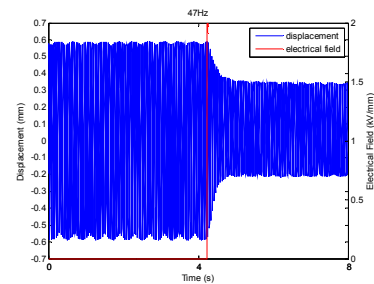
Fig. 17 Response using the fuzzy controller at 47 Hz (Turn on at 4.2 sec.)
