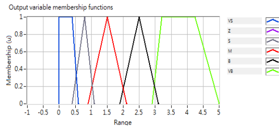
Fig. 11 The membership functions for the output
