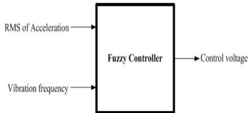
Fig. 8 The structure of the proposed fuzzy controller
