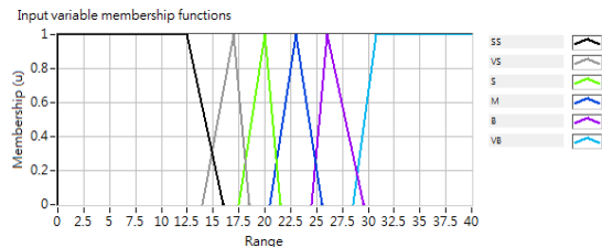
Fig. 10 Membership functions for the second input
