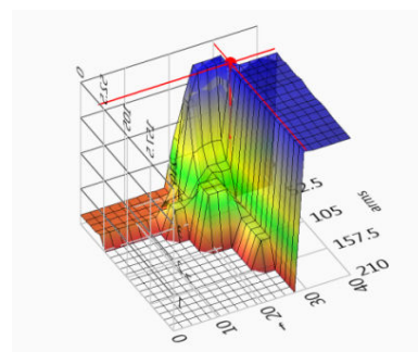
Fig. 12 The input-output mapping relation of the fuzzy controller
