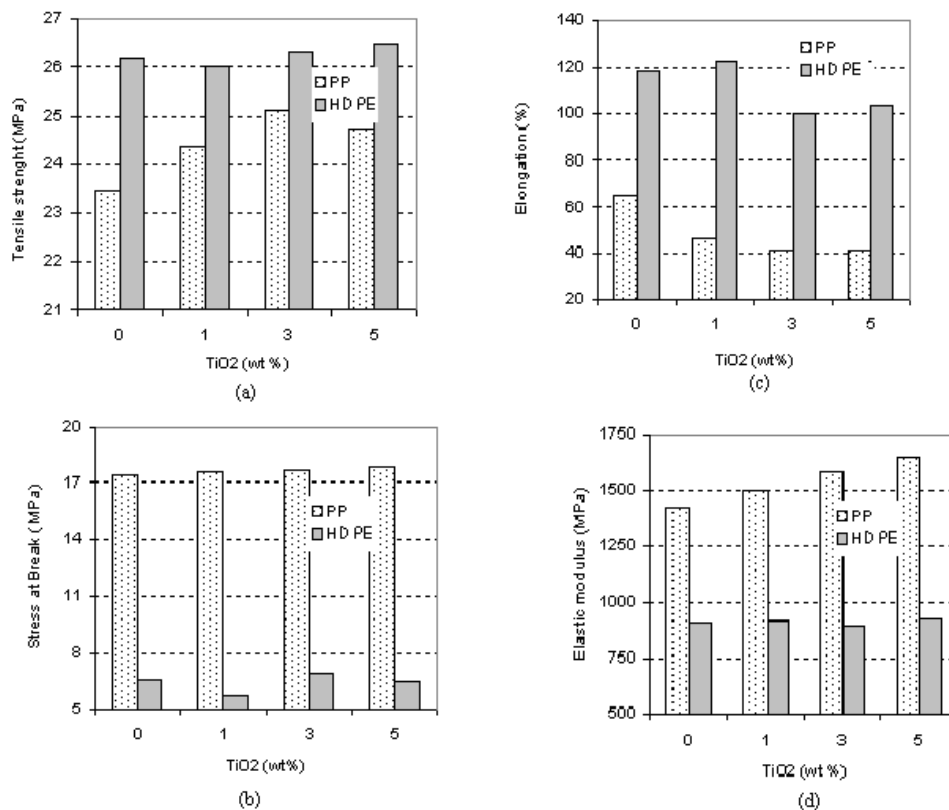
Fig. 4 Mechanical properties of nano \text{TiO}_2 reinforced PP and HDPE injection moldings obtained from tensile test
