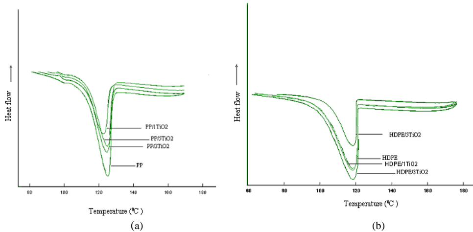
Fig. 3 DSC cooling scans of the \text{TiO}_2 reinforced PP (a) and HDPE (b) composites
