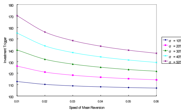
Fig. 5. The Mean-Reverting Effect under a Mean-Reverting Process
