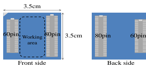
Fig. 5 Brief layout of a sensor module
