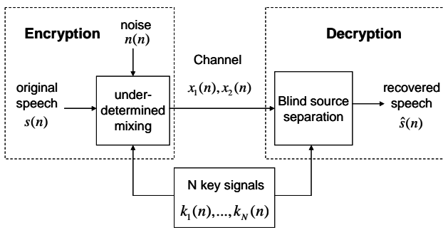
Fig. 1 Encryption scheme based on blind source separation
