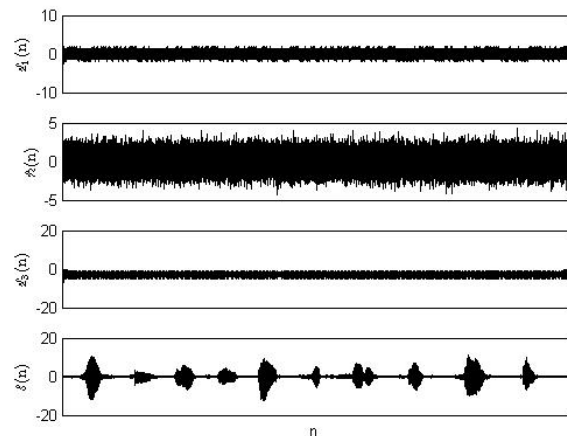
Fig. 4 Decrypted signals
