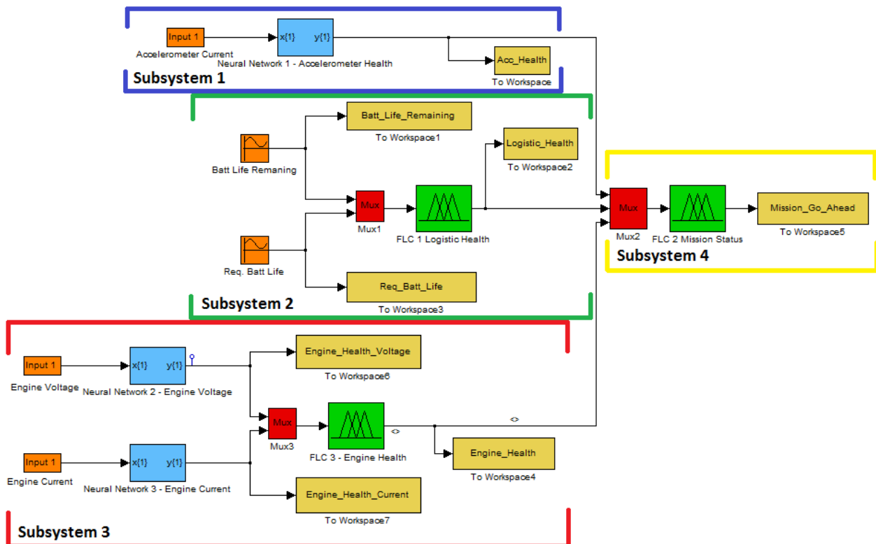
Fig. 3 Simulation Model
