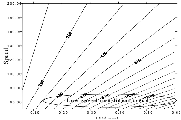
Fig. 1 Contours of cutting speed-feed rate-roughness interrelation
