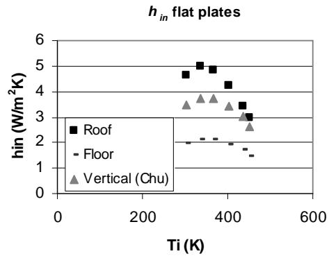
Fig. 5. Flat plate h_{in} vs car body temperature
