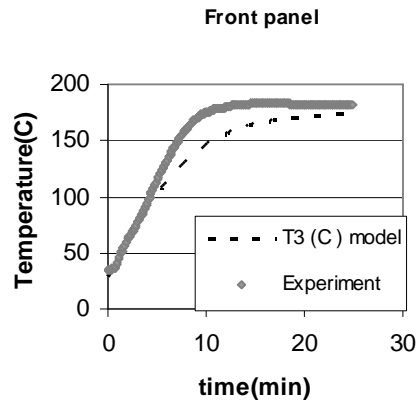
Fig.8. Front side, car body temperature vs time
