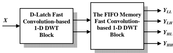
Fig. 8 The FIFO-based 2-D DWT fast convolution-based block diagram
