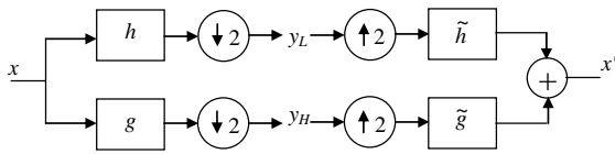
Fig. 2 Signal analysis and reconstruction in DWT
