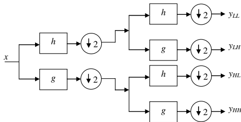
Fig. 3 Two-level multi-resolution wavelet decomposition
