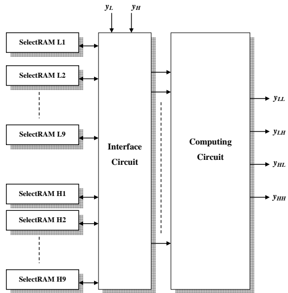
Fig. 7 The SelectRAM 1-D DWT fast convolution-based block diagram
