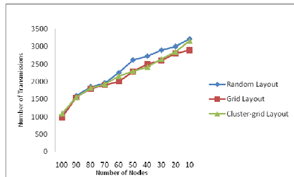
Fig. 3 Alive nodes with respect to transmissions.
