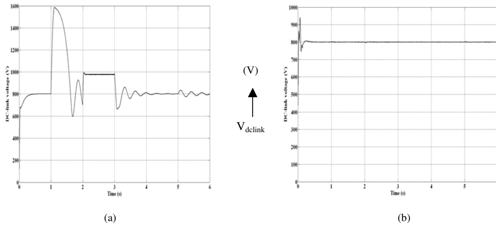
Fig. 4. Response of dc-link voltage
