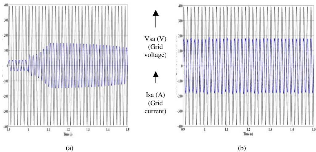
Fig. 5. Grid voltage and current with Transition from unity pf to leading pf (Time: X-axis 0.9~1.5 sec,
