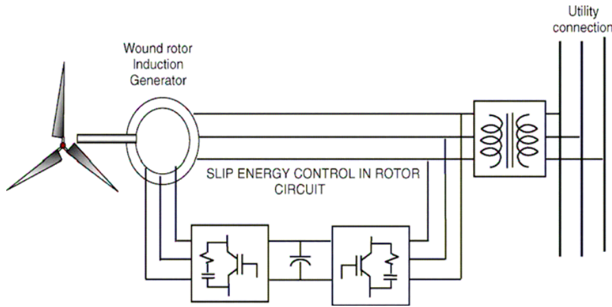
Fig.1: DFIG with bi-directional pulse with modulation converter
