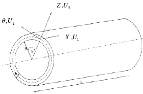
Fig. 1 Geometry of a cylindrical shell
