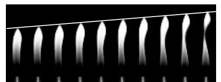
Fig. 2 Diffusion flame in straight pipe burner at 200 mlpm methane flow rate, which appears to be steady. Time interval between two consecutive images is 0.003 seconds.
