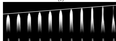
Fig. 3 Diffusion flame in a contoured burner at 310 mlpm methane flow rate, which exhibits intermittent flickering. (a) and (c) shows intermittently flame flickering with different amplitudes and (b) shows steady flames. Time interval between two consecutive images is 0.003 seconds
