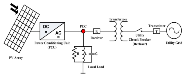
Fig. 9 Topology of power line carrier communication control with transmitter (T) and receiver (R) added to the system.
