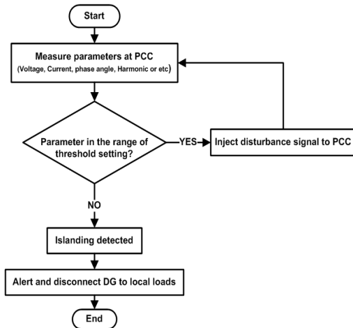
Fig. 8 The flow chart describing the process of a hybrid islanding detection procedure.
