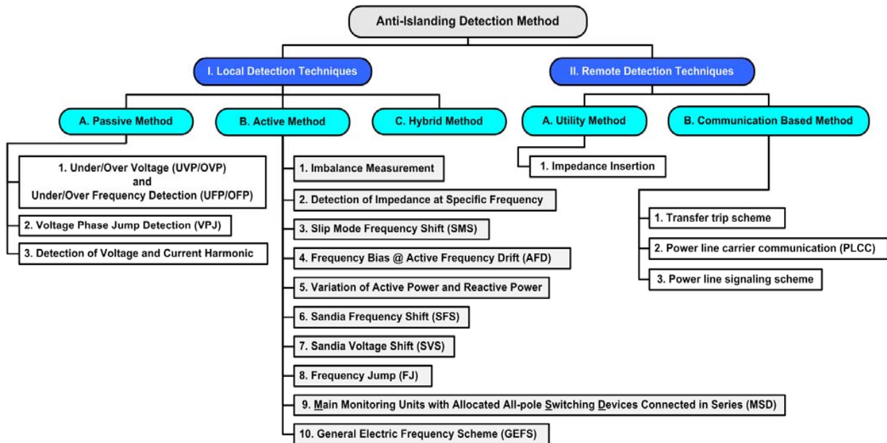
Fig. 2 The classification of anti-islanding detection techniques
