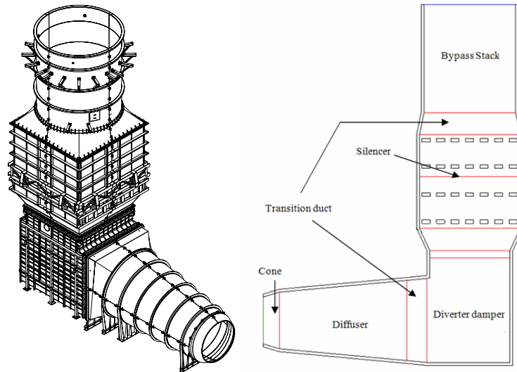
Fig. 1 The 3D drawing (Left) and 2D model (Right) of the exhaust system
