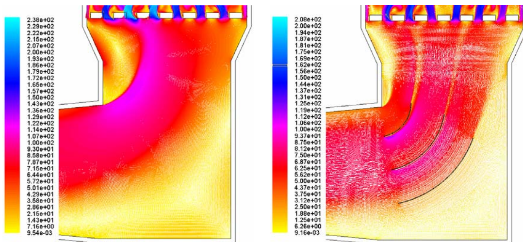
Fig. 4 Comparison of flow pattern in diverter box (velocity vectors m/s)
