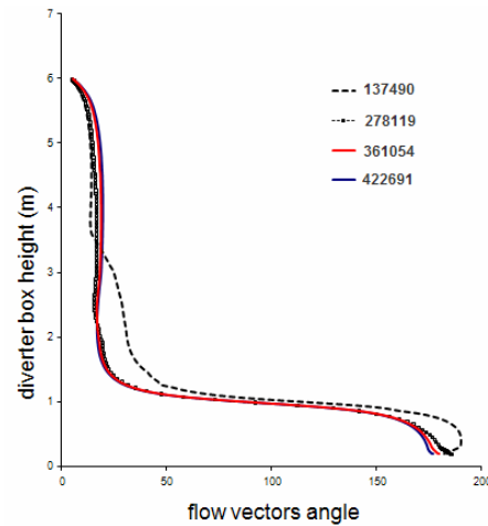
Fig. 2 Grid independency checkout
