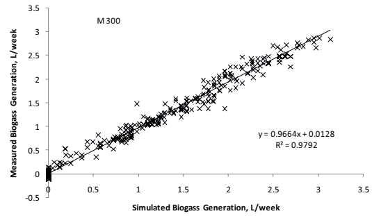
Fig. 5 Linear regression between modeled and actual data for ANFIS sub-models: M-50, M-100, M-150, M-200, M-250, and M-300
