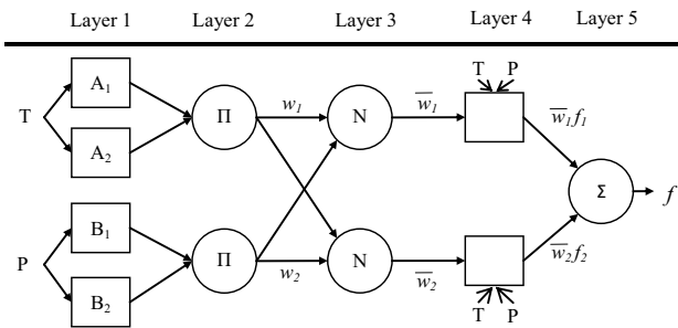
Fig. 3 Architecture of a minimized ANFIS model
