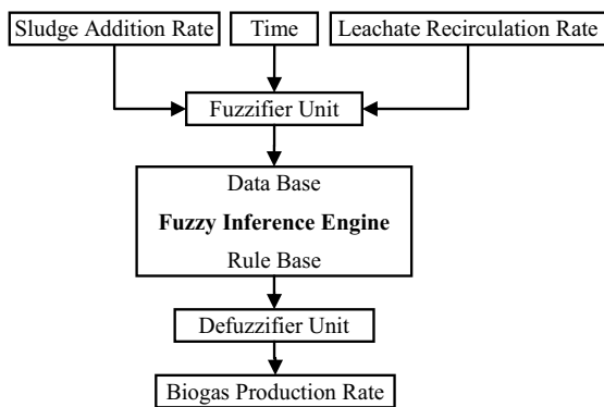
Fig. 1 Typical structure of a fuzzy logic controller
