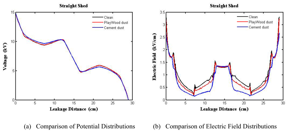
Fig. 11 Under Uniform Contamination Conditions without Water Droplets
