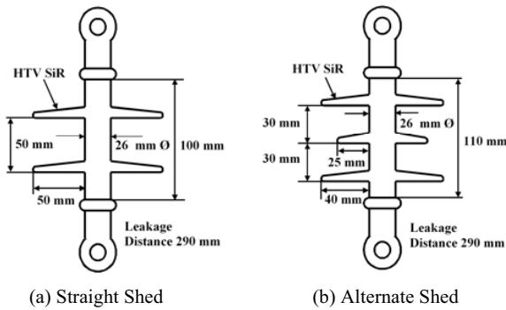
Fig. 2 Test Specimens.
