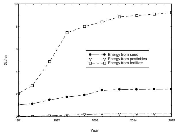
Fig. 4 Simulated results of energy input [GJ/ha] from seed, chemical fertilizer and pesticide in basic mode for the period of 1981-2025
