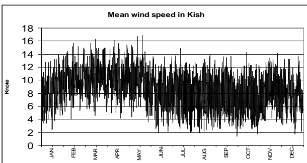
Fig. 4 Daily Wind Speed in Kish Island
