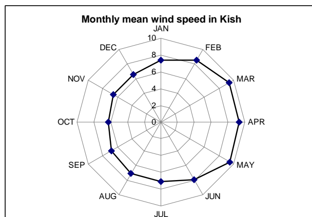
Fig. 1 Monthly wind speed in Kish Island
