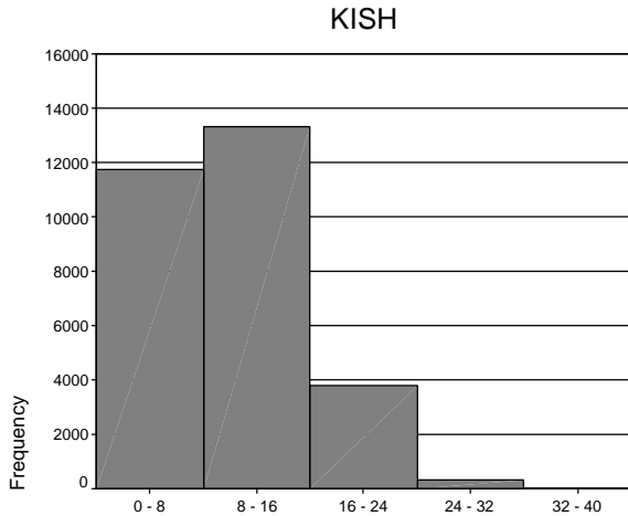
Fig. 2 Wind Speed Histogram in Kish Island
