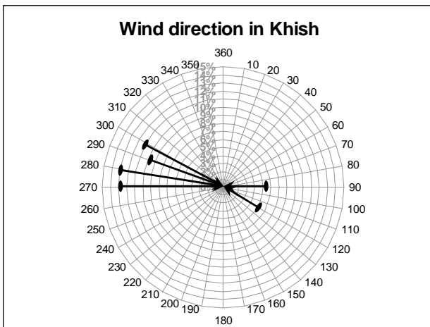
Fig. 3 Wind Direction in Kish Island
