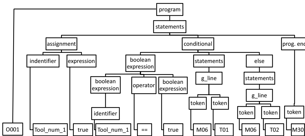
Fig. 5. AST for the EGCL example program in Figure 4.
