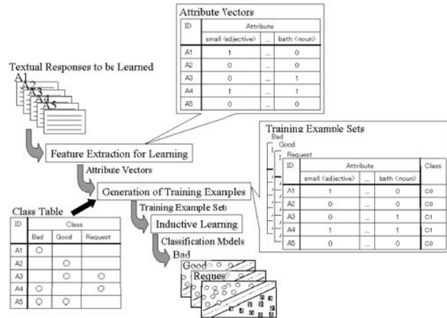
Fig. 1. Learning phase
